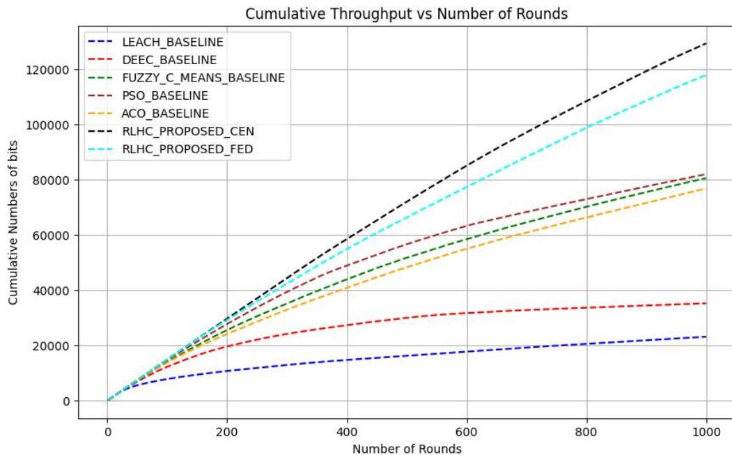
Figure 6.4 Cumulative Throughput
